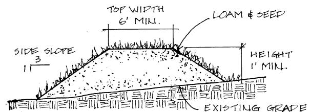
Typical diversion berm
