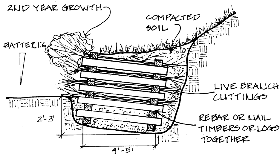
Live cribwall
