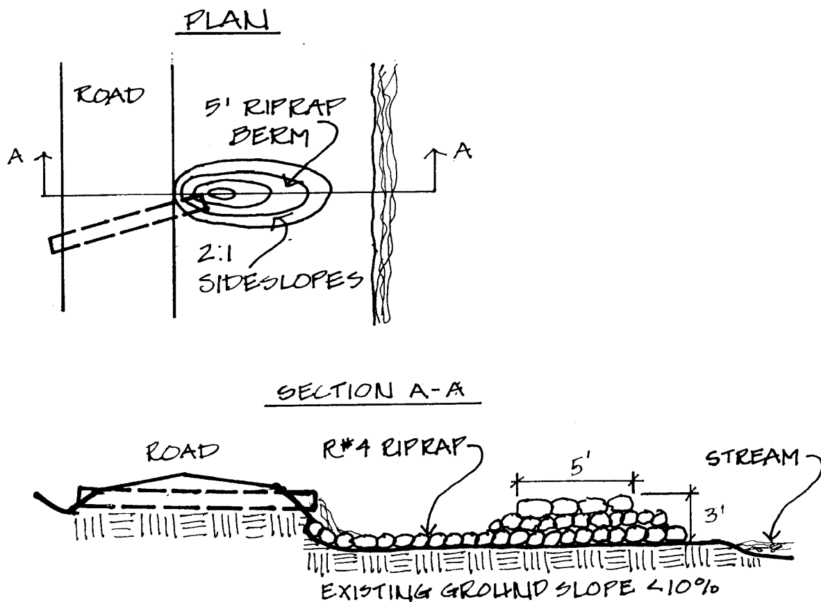
Cross section of a splash/plunge pool
