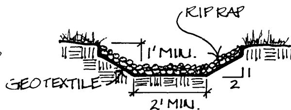
Riprap conveyance channel profile
