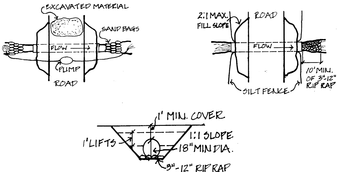
Culvert installation details
