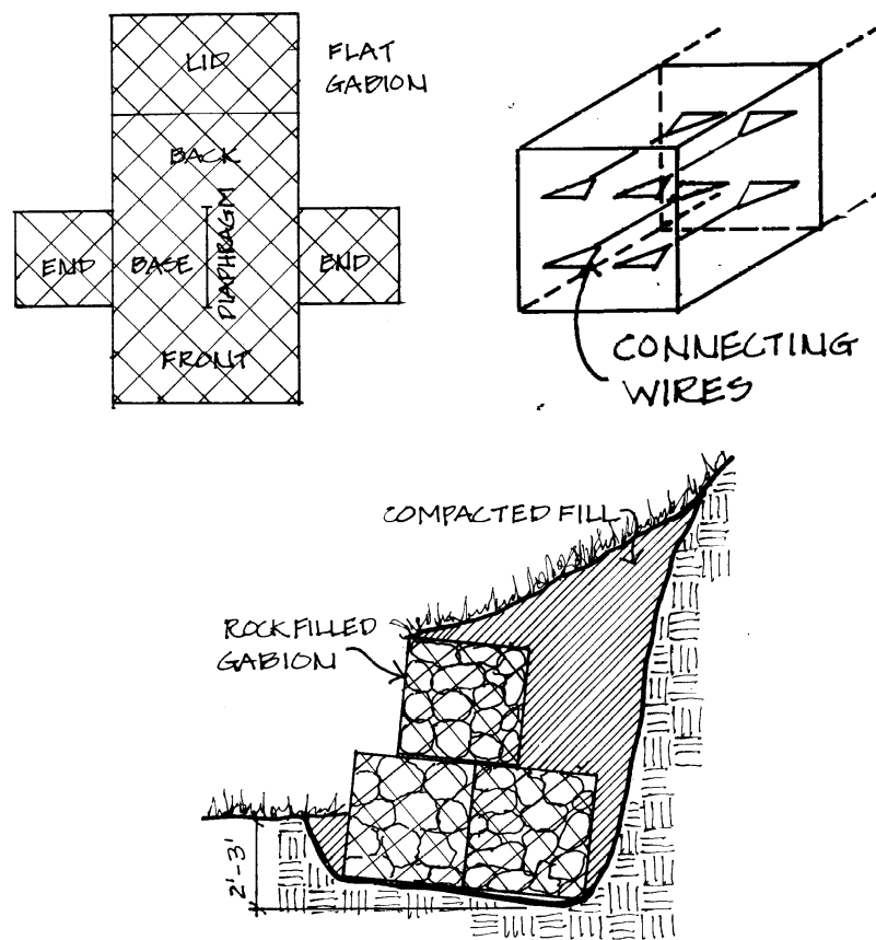
Gabion wall
