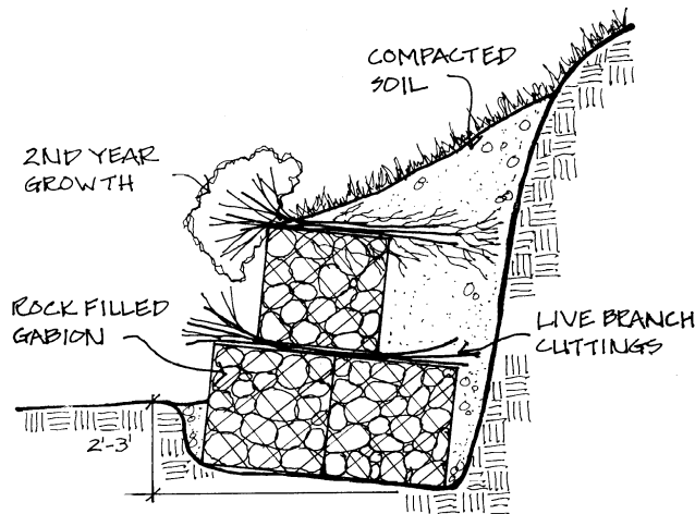
Vegetated gabion
