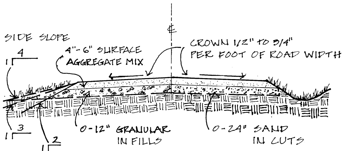
Typical crown and road profile (1 inch=8 feet)
